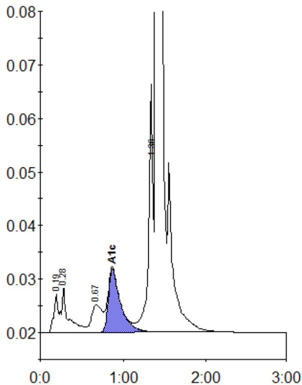
Peak table - ID: 10483162
